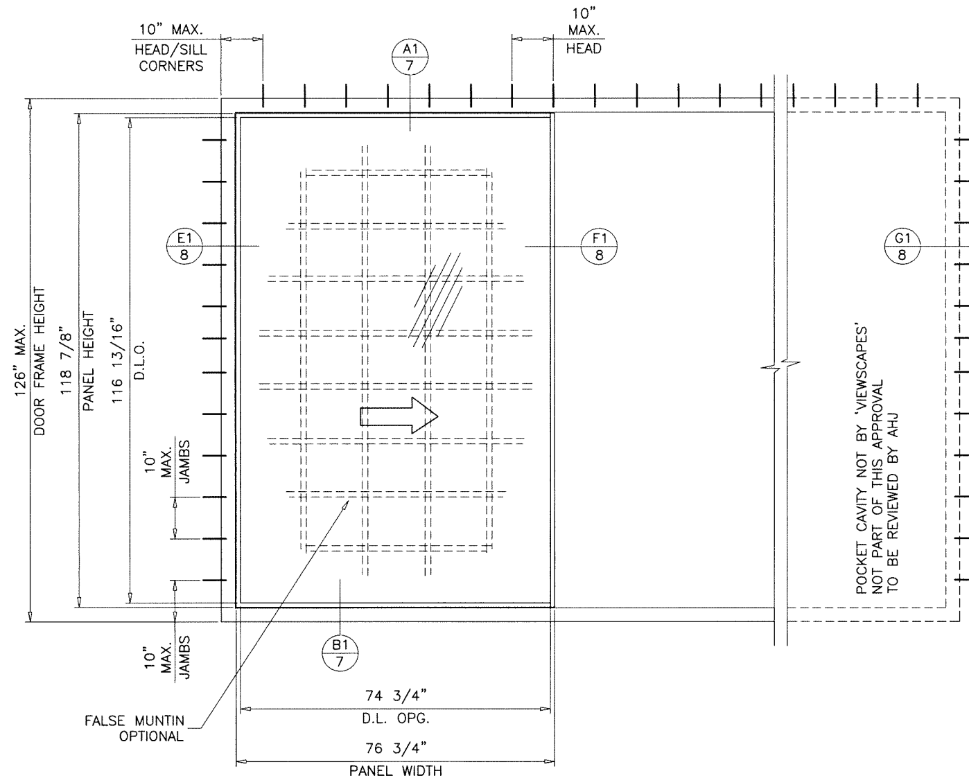
TYPICAL ELEVATION TESTED UNIT
