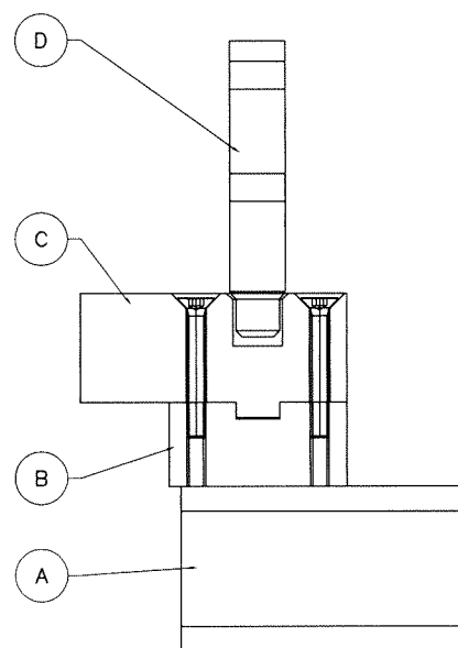
BOTTOM BRACKET
