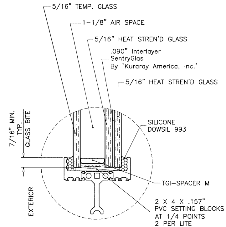
GLAZING DETAIL 2-1/8" OVERALL INSUL. LAM. GLASS
